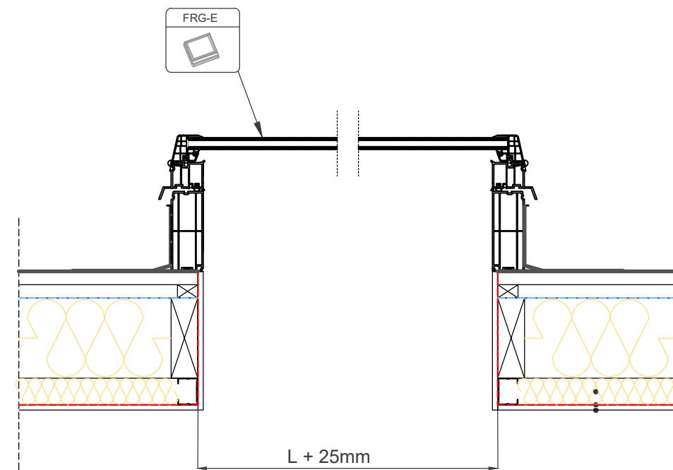
Section B-B' 1:10
