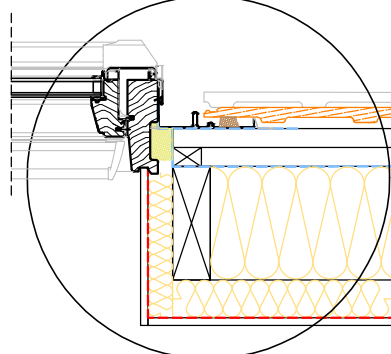
Section B-B' 1:10
