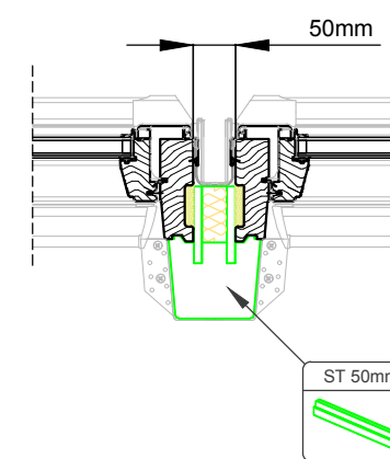
Detail B 1:5
