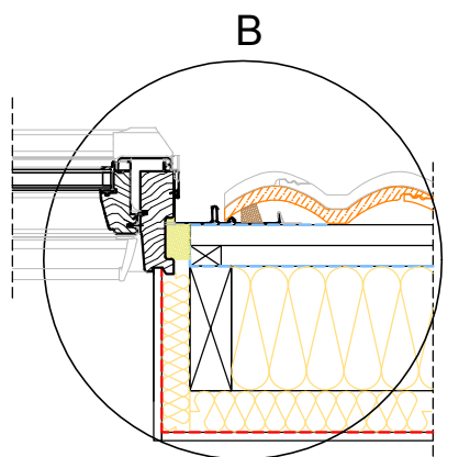
Section B-B' 1:10
