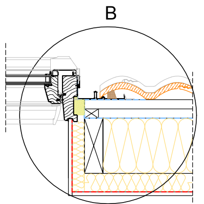
Section B-B' 1:10
