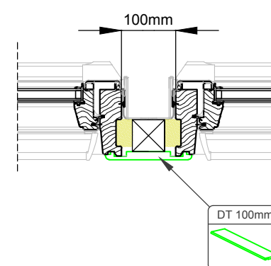
Detail B 1:5
