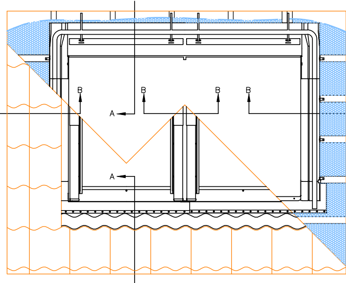
INDICATIVE SECTIONAL VIEW
