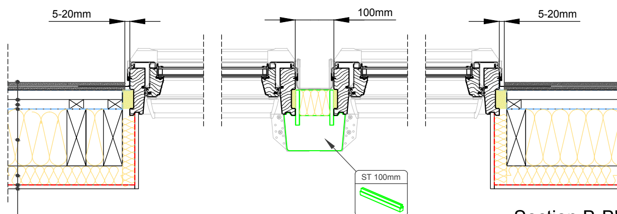
Section B-B' 1:10
