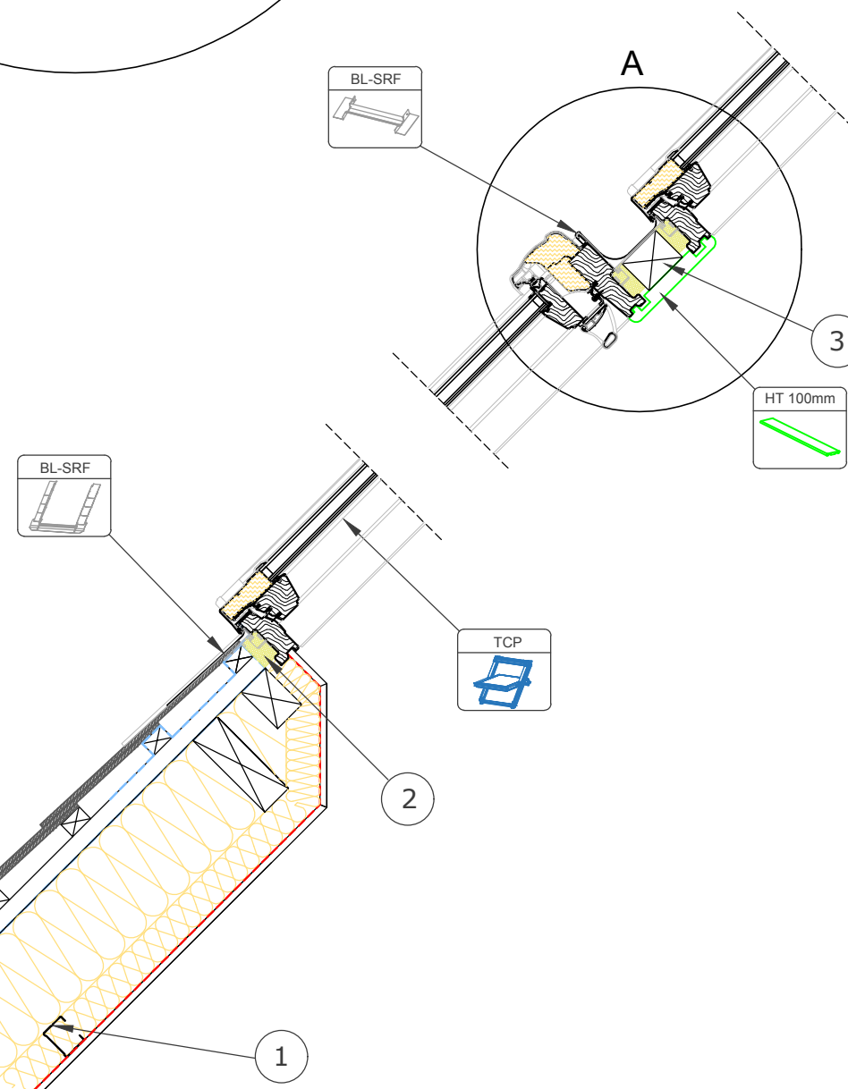
Section B-B' 1:10
