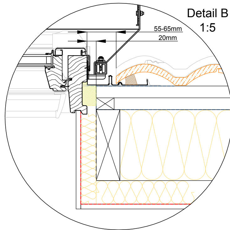
INDICATIVE SECTIONAL VIEW
