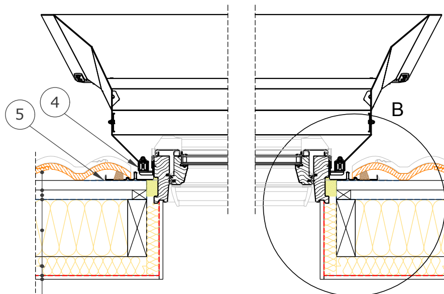
Section B-B' 1:10
